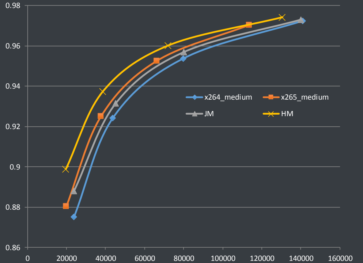
SSIM vs Bitrate
