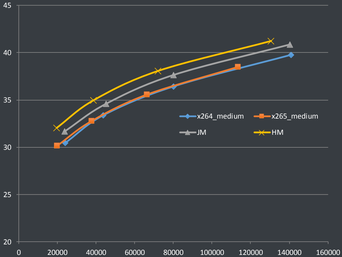
PSNR vs Bitrate
